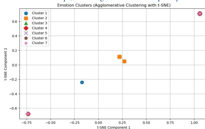
Figure 5: Agglomerative Clustering with t-SNE
