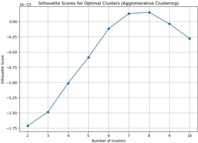
Figure 3: Elbow Method
