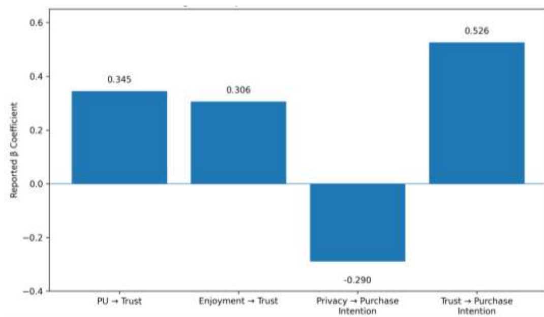
Figure 2. Effects from the Published PLS-SEM Study
